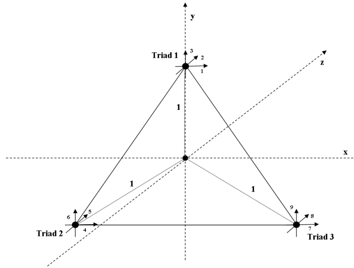
Figure 3.7: 3 Accelerometer Triads
